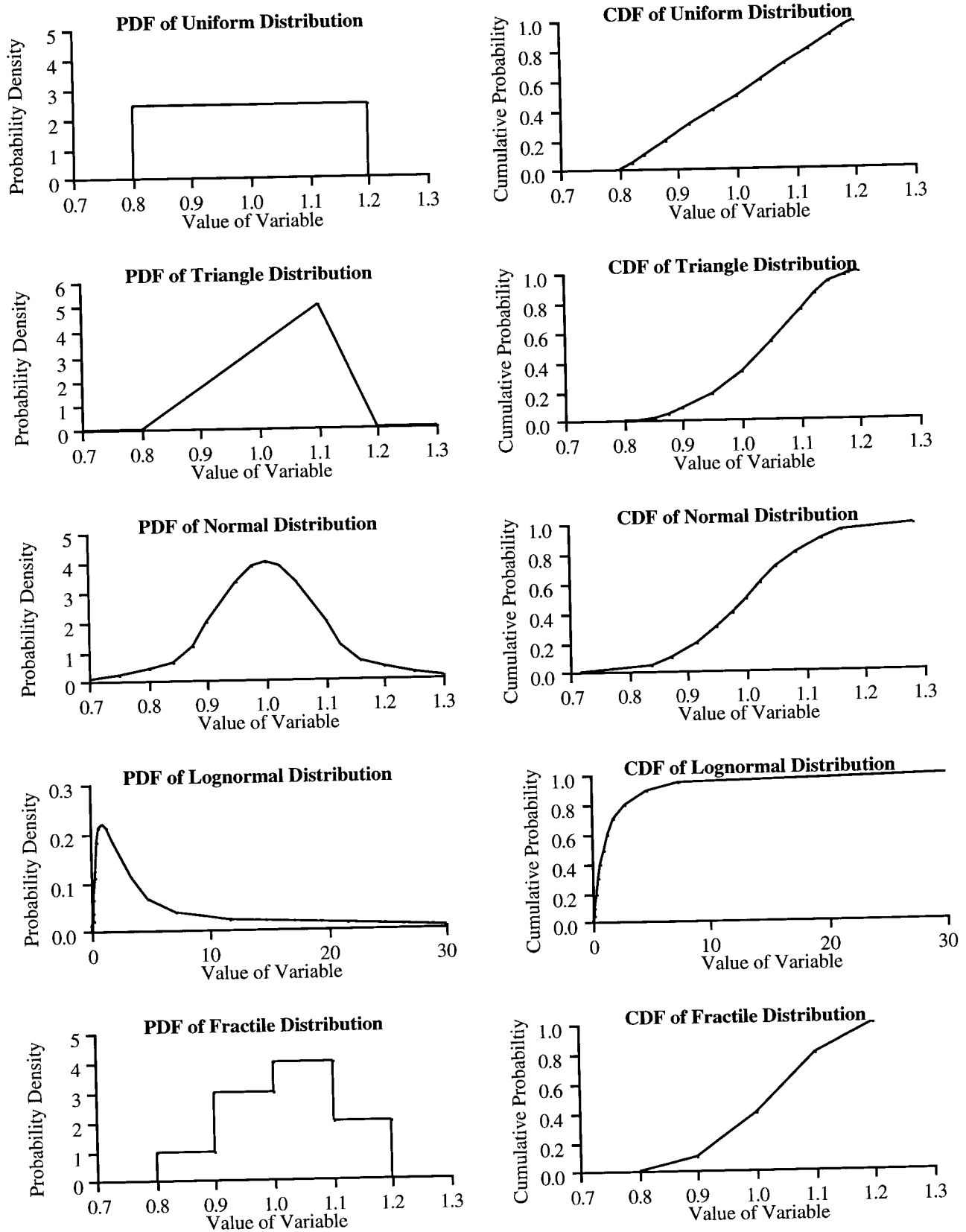
Figure 2. Some Types of Probability Distributions.
