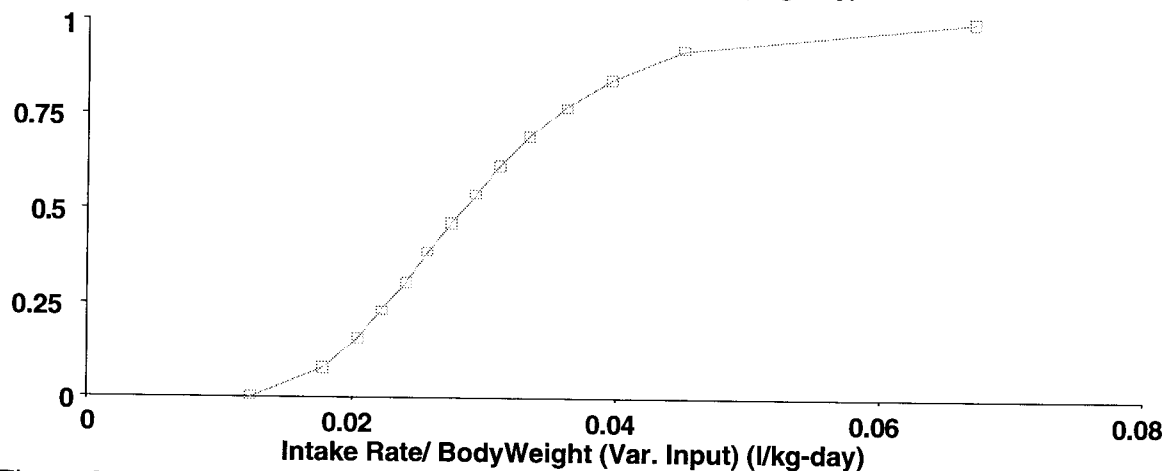
Figure 8. Model input frequency distribution for variability in intake rate per unit body weight.
