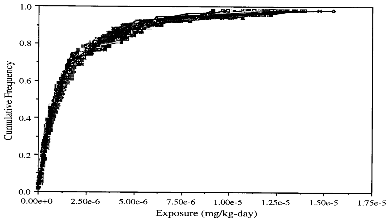
Figure 12. Results of a two-dimensional simulation of variability and uncertainty in a hypothetical exposure model.
