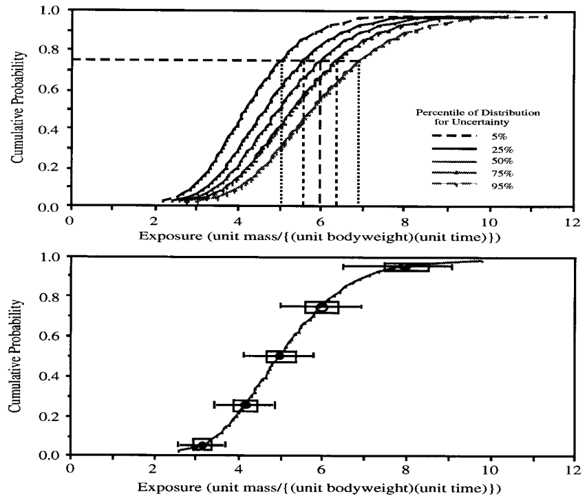
Figure 15. Use of error bars to represent uncertainty in exposure levels for specific fractiles of the population distribution: A simple example.
