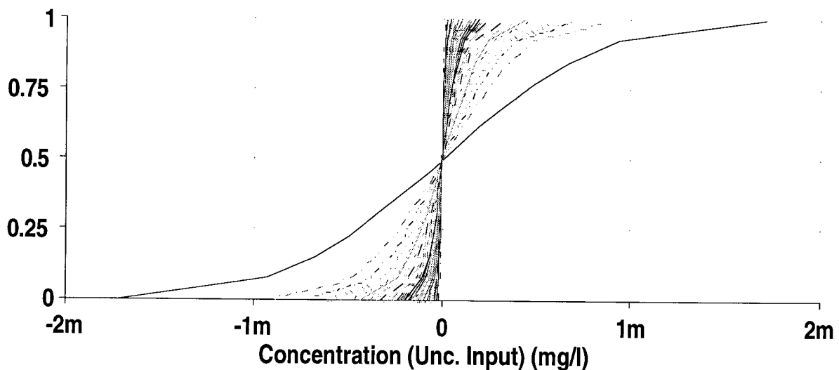
Figure 11. Family of Probability Distributions for Uncertainty in Concentration Associated with Each Individual in the Population.
