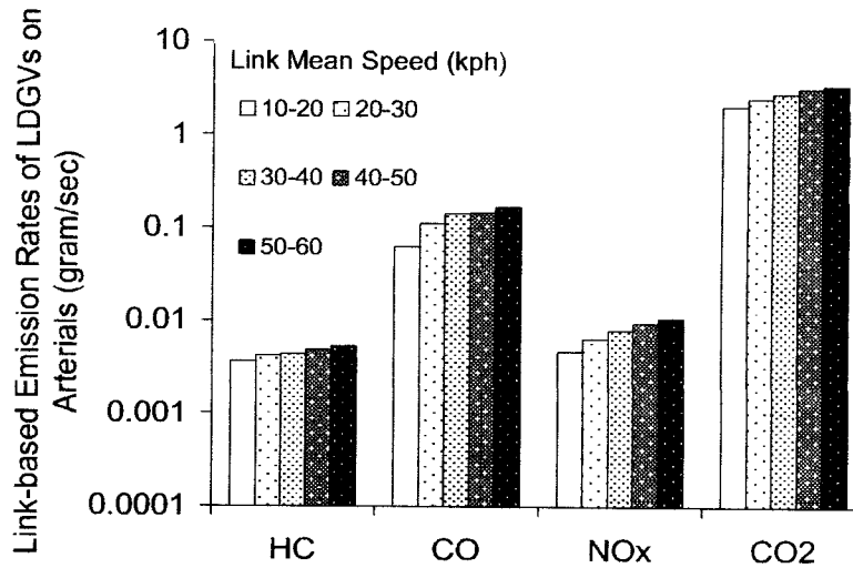
Figure 2 Examples of Emission Factors for Light-duty Gasoline Vehicles (LDGVs) in Baseline Scenario
