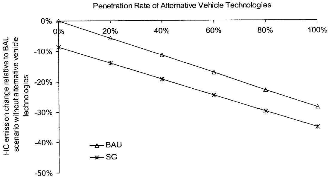
Figure 3 Sensitivity of HC Emissions from Light-duty Vehicle Fleet to Total Penetration Rate of Alternative Vehicle Technologies
